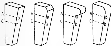
FIG. 255. SIMPLE FORMS OF KEYS.
